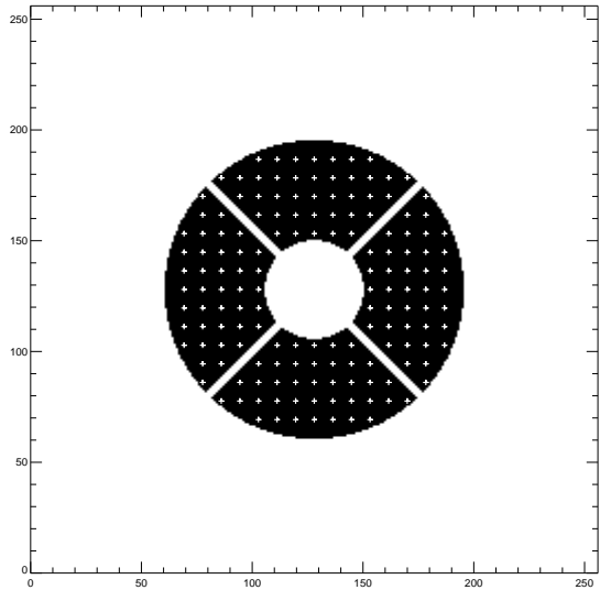
FIG. 2.— Model for the geometry of the HST/NICMOS pupil and location of the sample points for the determination of the Ker-phase relations. The 156 sample points of the pupil fall on a regular square grid with a step of 1/16^{th} of a pupil diameter that do not intersect with the central obstruction or the spider arms.
