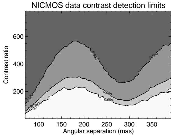
FIG. 5.— Level of confidence in the detection of a companion from the analysis of the HST/NICMOS data with the Ker-phase algorithm. A darker color indicates a region of lower confidence level. Three levels are highlighted: the 90%, 99% and 99.9% confidence levels. At angular separation 0.5 \lambda/D (i.e. 80 mas at \lambda = 1.9 \mu\text{m} ), a contrast limit better than 50:1 is possible at the 99% confidence level.
