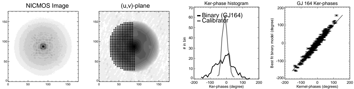
FIG. 3.— From left to right: example of a narrow band (F190N) NICMOS1 image used for this work, visualized with a non-linear brightness scale; The Fourier transform of this image. The 366 sample points for the phase in the Fourier domain are overlaid; A comparison of histograms of the 288 Ker-phases calculated using the relations identified in Section 2.1. By design, the Ker-phases calculated from images of a single star are expected to be zero within uncertainty: the corresponding histogram (gray curve) confirms this expectation. In comparison, the Ker-phase histogram of the binary (dark curve) appears significantly larger. The same GJ164 Ker-phases plotted against the model of a binary star that best fits the data achieve to convince of the presence of a companion in the data.
