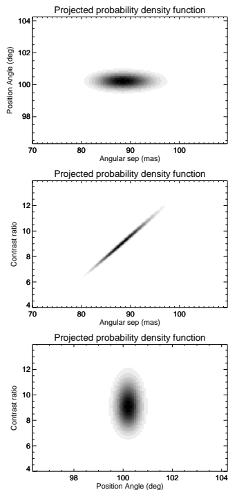
FIG. 4.— To determine confidence intervals for the parameters of the binary, a likelihood analysis comparable to the one presented by for closure-phase was performed. These panels show the three projections of the likelihood function in the region of best fit. Except for the expected correlation between angular separation and contrast ratio for a detection within 1 \lambda/D , the solution is unambiguous and well constrained, demonstrating the elegance of the Ker-phase approach.
