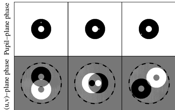
FIG. 1.— Iterative process for the determination of the transfer matrix \mathbf{A} . The top row shows the sub-aperture of the full 2D pupil (circular aperture with 30% central obscuration) where a phase offset is applied (three cases are represented). The bottom row shows the resulting distribution of phase in the Fourier plane. The overlaid dashed-line circle in the bottom row marks the cutoff spatial frequency of the transfer function.
