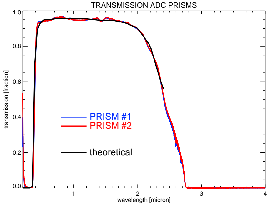
Figure 6. The transmission of the ADC unit as a function of the wavelength. The measured transmission for both prisms match very well the theoretically expected transmission based on the used glass types.
