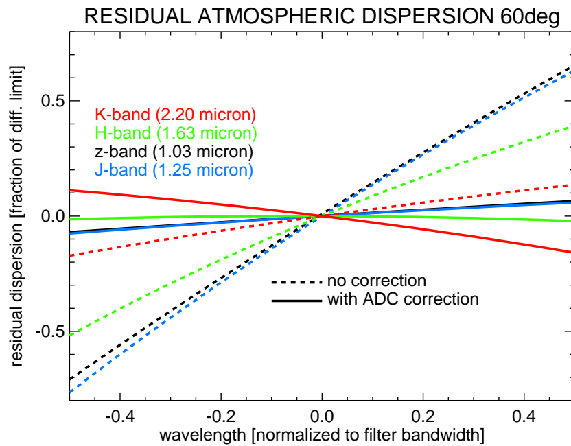
Figure 3. The atmospheric dispersion as a function of the normalized wavelength within each filter of IRCS for a zenith distance of 60 deg. Without the correction by the ADC (dashed lines), the atmospheric dispersion can reach up to 60% of the diffraction limited PSF. This means that the PSF will be elongated by a factor of 1.6 along the elevation axis. With the correction by the ADC (solid lines), the linear term of the dispersion is gone and a small quadratic residual dispersion remains. The rotation angle of the ADC prisms are adjusted to achieve the optimal correction for all filters simultaneously. Therefore the dispersion in K-band has still a small residual linear component.
