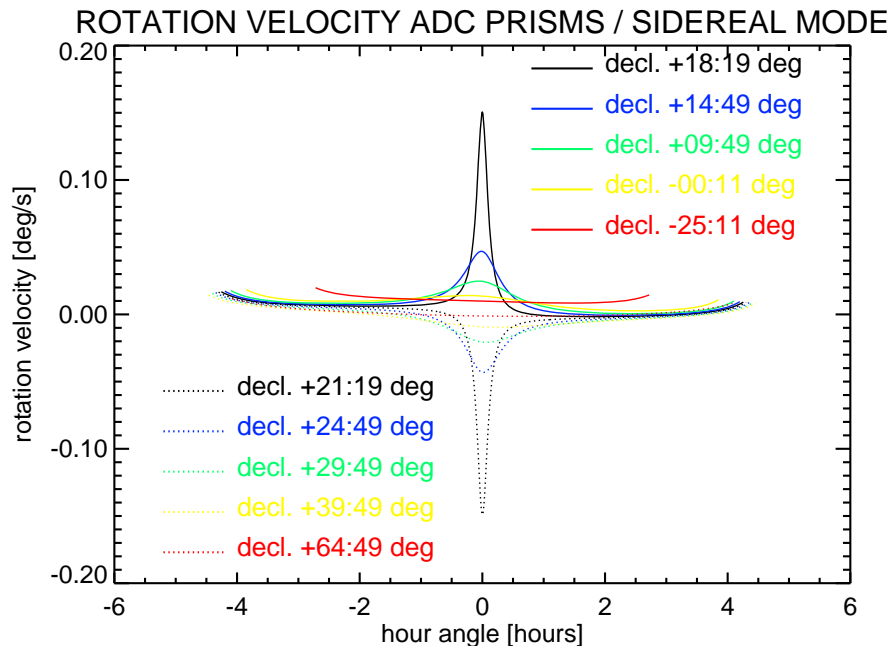
Figure 9. The rotation velocity of the ADC prisms as a function of the hour angle of the object. The different colors correspond to different values of the declination of the objects.
