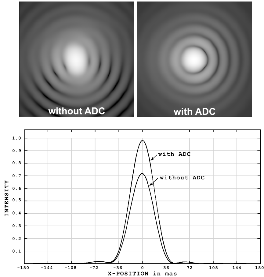
Figure 4. The PSF in H-band with and without the correction of the atmospheric dispersion by the ADC unit. This is the internal PSF of the AO system only, no central obstruction or spiders of the telescope have been taken into account. The field-of-view is 2.3 \times 2.3 arcsec. Without the ADC unit, the internal Strehl-ratio drops to 72% and is restored to 98% with the ADC unit.
