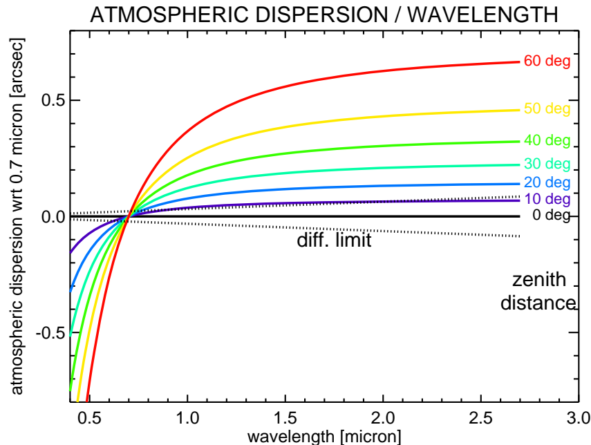
Figure 1. The atmospheric dispersion as a function of the wavelength. The various curves correspond to different zenith distances.
