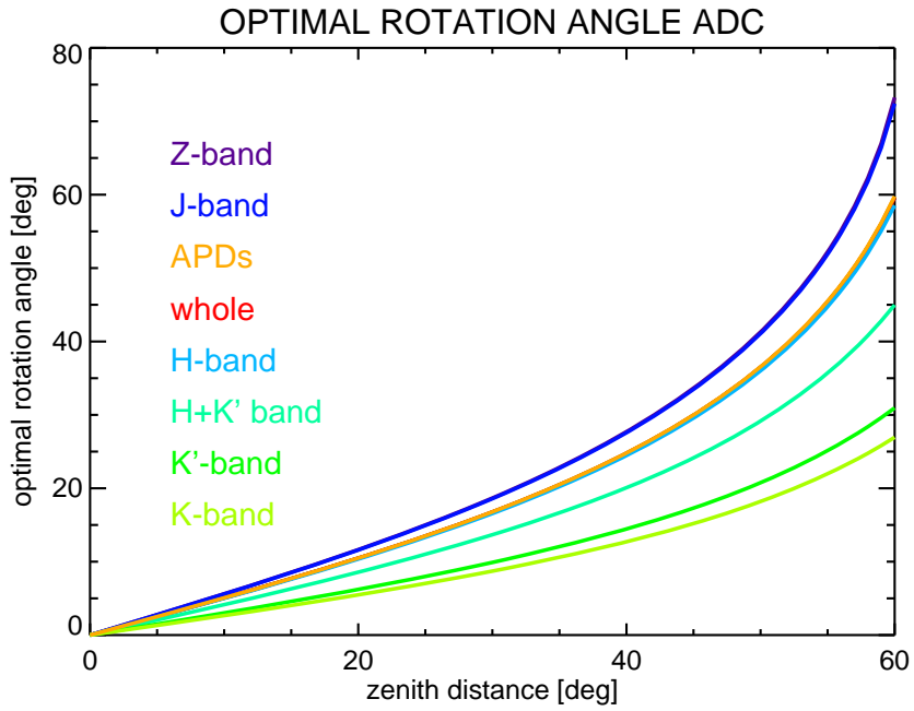
Figure 5. The optimal rotation angle of the two prisms with respect to each other for the various science filters used, as a function of the zenith distance. "Whole" means that the rotation angle was optimized for all filters simultaneously.
